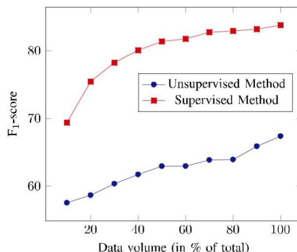
Fig. 9. F_1 -scores for different sizes of the training set (% of 3000 sentence).
