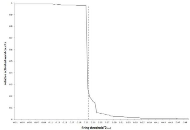
Fig. 4. Graph displaying the relative activated word counts for different values of firing threshold \tau_{food} together with the threshold chosen by the heuristic.
