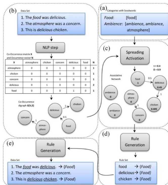
Fig. 2. Example flowchart of the unsupervised method. [the steps are:
