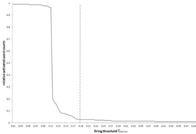
Fig. 3. Graph displaying the relative activated word counts for different values of firing threshold \tau_{service} together with the threshold chosen by the heuristic.
