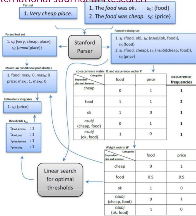
Fig. 5. Example flowchart of the supervised method.
